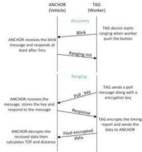
Figure4.Message exchange during the discovery and ranging phases
