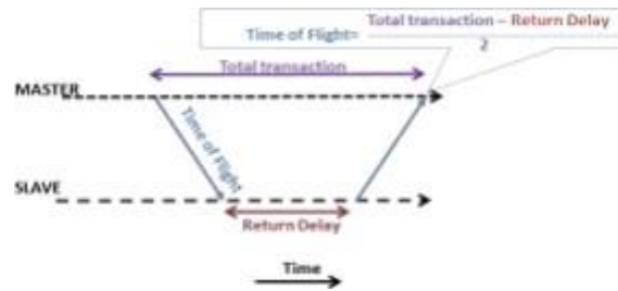
Figure3.TimeofFlighttimedomainrepresentation
