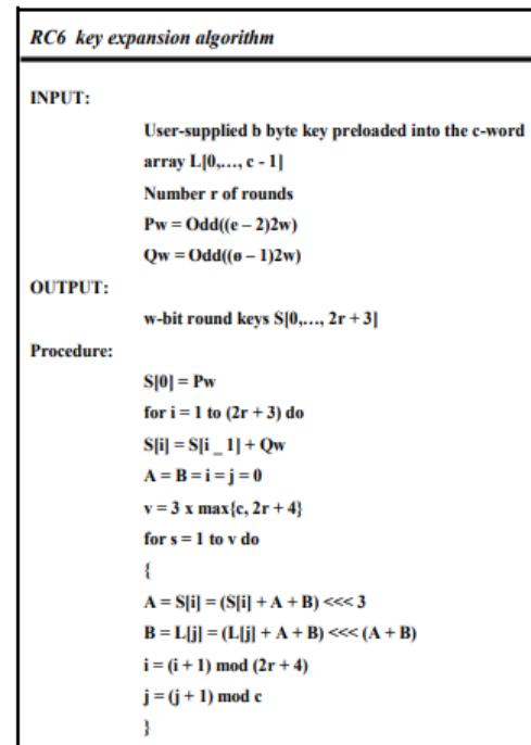
Fig 5: Key Expansion Algorithm of RC6
