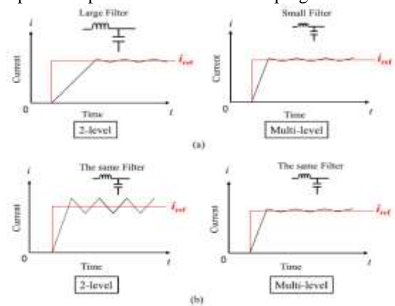
Fig. 3. Example of current waveforms in step response depending on the number of output levels and output filter of converters. (a) When both filters are specifically designed for same ripple of output current. (b) When both filters have the same parameters.
