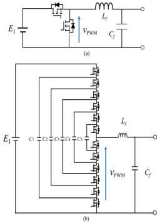
Fig.2. Circuit configurations of power flow controllers. (a) Two-level topology. (b) Multi-level topology (seven-level case).
