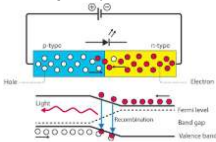
Figure.7: Working of LED
