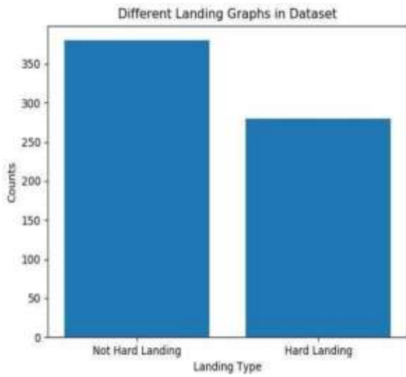
Fig.2. Loading Dataset.
