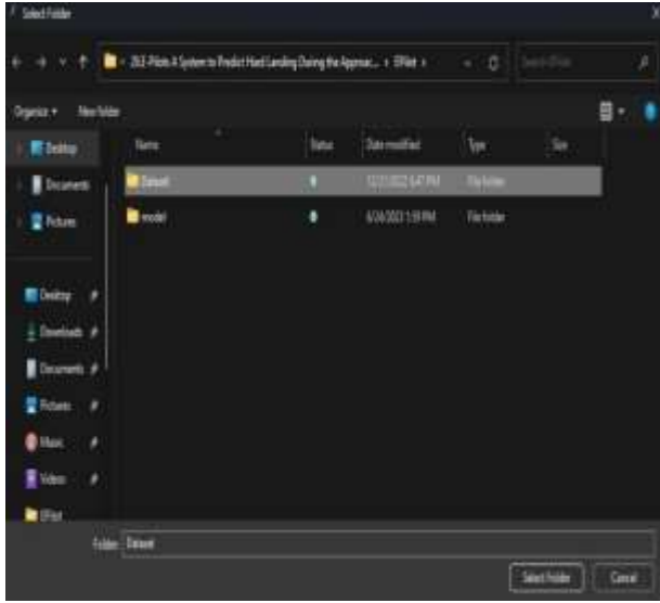
Fig.2. Loading Dataset.
