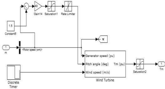
Fig 2 simulation circuit
