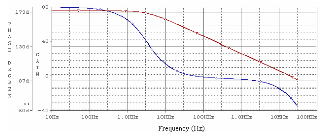
Fig.4 Gain and phase curve
