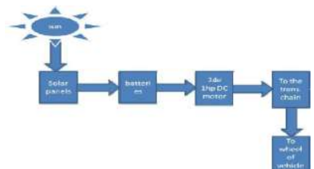
Fig.2 Basic block Diagram Representation of Solar vehicle.
