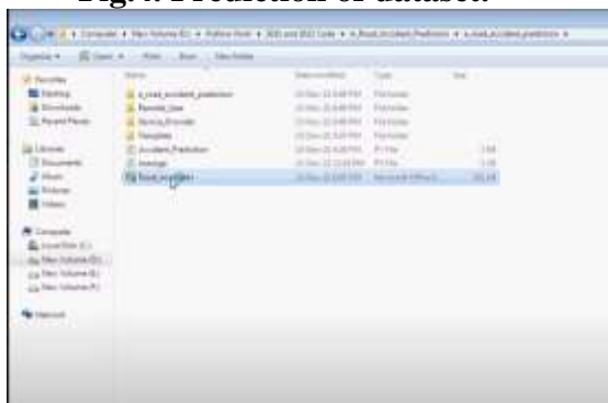
Fig.5. Dataset details.
