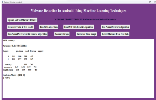
Fig.3. Algorithm applied.
