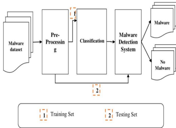
Fig.2. System Diagram.
