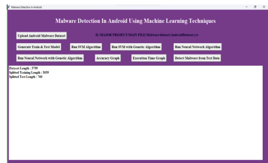
Fig.2. Data loaded.
