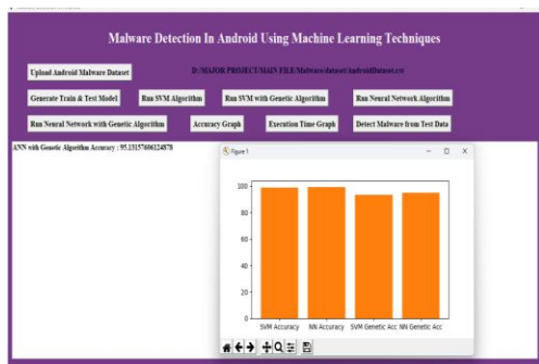
Fig.5. OUTPUT graphs.
