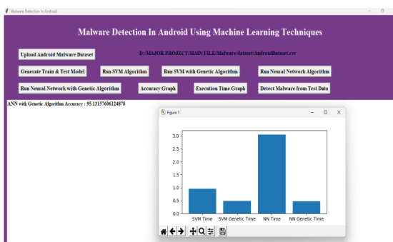
Fig.5. OUTPUT graphs.
