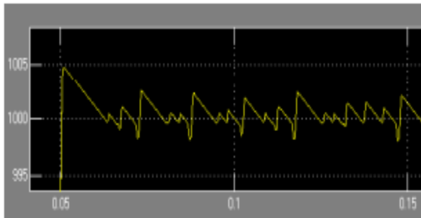
Figure (20) Zoomed speed response of SRM with P controller for 1000rpm on no load showing overshoot
