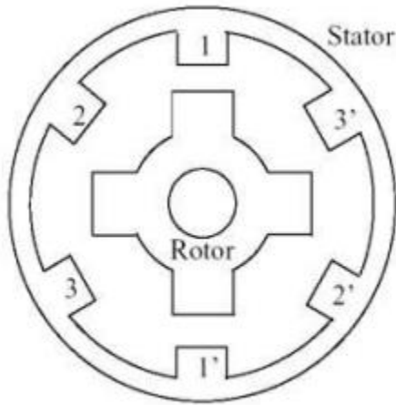
Figure (1) Switched Reluctance Motor.
