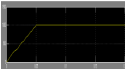
Figure (25) speed response of SRM with PI controller for 1000rpm on no load
