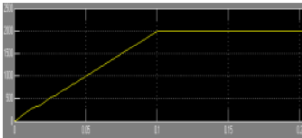
Figure (21) speed response of SRM with P controller for 2000rpm on no load
