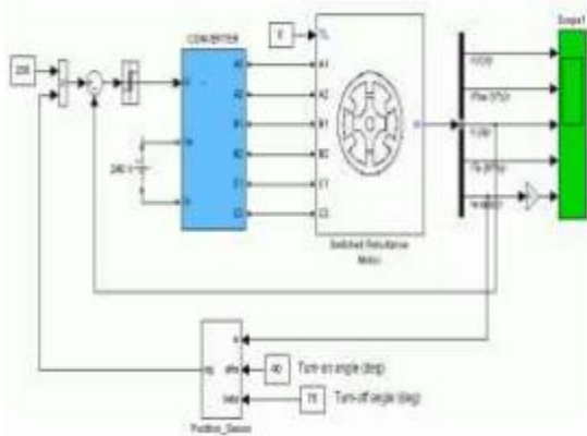
Figure (6) MATLAB Simulink modeling of 6/4 SRM
