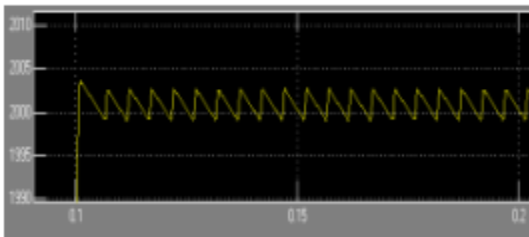
Figure (22) Zoomed speed response of SRM with P controller for 2000rpm on no load showing overshoot
