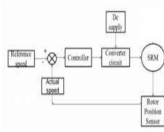
Figure (5) Block diagram of typical SRM control scheme [4].
