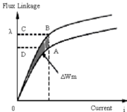
Figure (3) Flux Linkage Chart.
