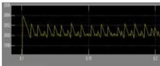
Figure (28) Zoomed speed response of SRM with PI controller for 2000rpm on no load showing overshoot
