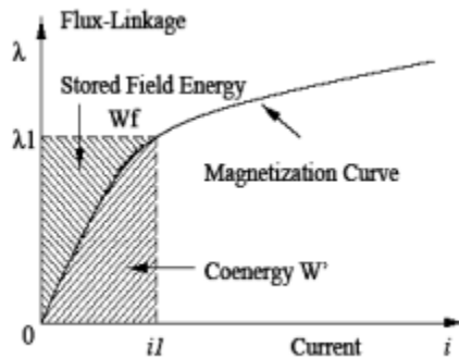
Figure (4) Energy Exchange.
