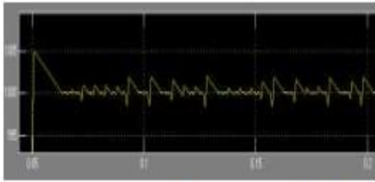
Figure (26) Zoomed speed response of SRM with PI controller for 1000rpm on no load showing overshoot
