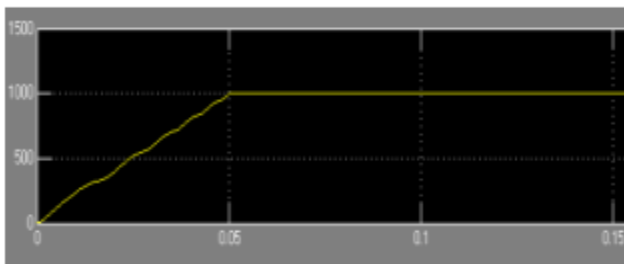
Figure (19) speed response of SRM with P controller for 1000rpm on no load
