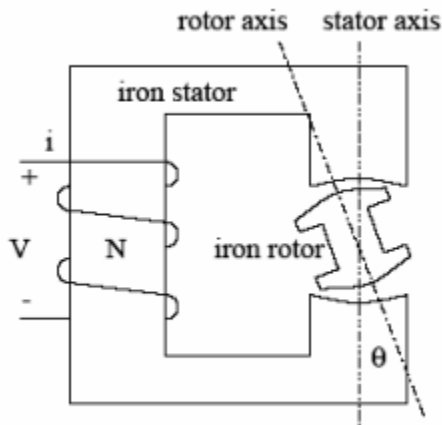
Figure (2) Single Phase SRM.
