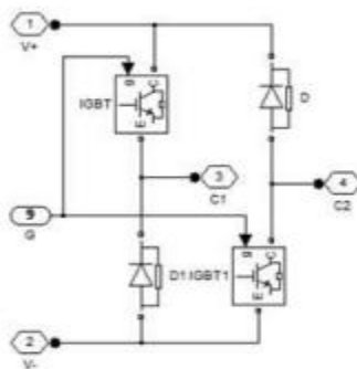
Figure (10) per phase converter, showing the switching devices
