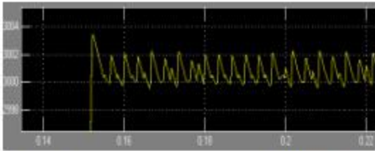
Figure (30) Zoomed speed response of SRM with PI controller for 3000rpm on no load showing overshoot
