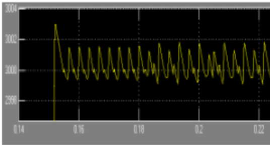
Figure (24) Zoomed speed response of SRM with P controller for 3000rpm on no load showing overshoot
