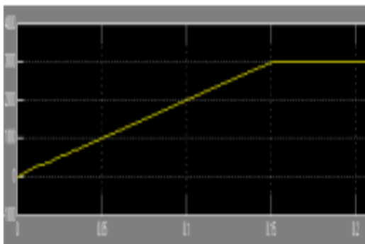
Figure (29) speed response of SRM with PI controller for 3000rpm on no load
