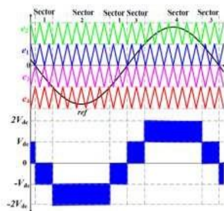
Fig. 7 LS-PWM scheme
