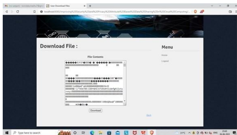
Fig 4.2 Encrypted Data
