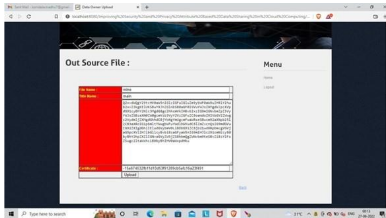
Fig 4.2 Encrypted Data
