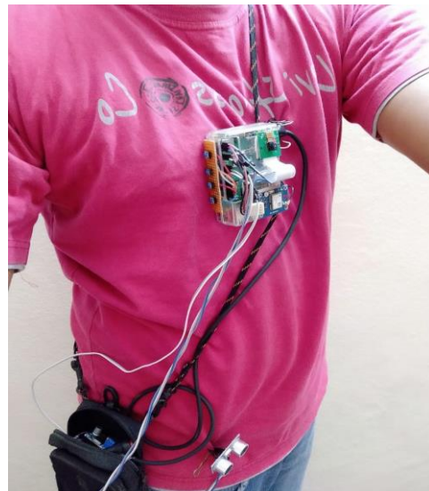
Figure 7: Implementation of Hardware Setup
