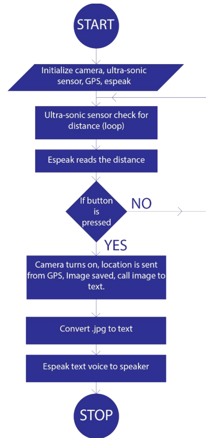
Figure 9: Flow Chart
