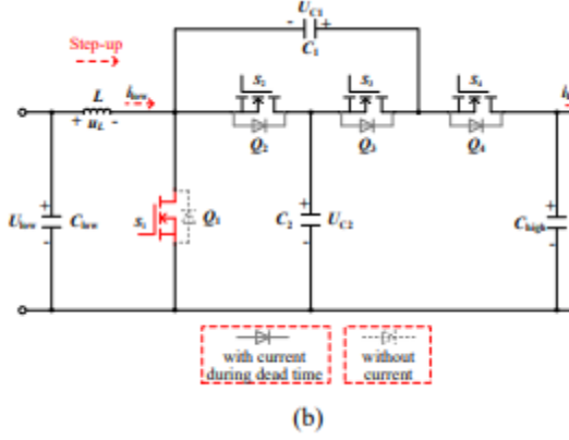
Fig. 4 Synchronous rectification operating principle for the proposed bidirectional converter. (a) Gate signals and dead time in the step-up mode. (b) Current-flow paths in the step-up mode.
