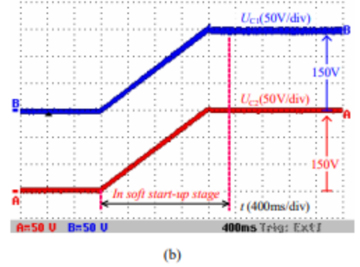
Fig. 10 Experimental results of the soft start-up. (a) The input voltage U_{low} and the output voltage U_{high} . (b) The voltages across C1 and C2 .
