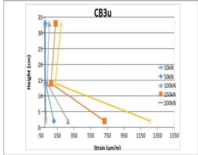
Figure 7: Position of Neutral Axial Versus Applied Load for CB3u
