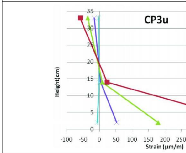
Figure 6: Position of Neutral Axial Versus Applied Load for CP3u
