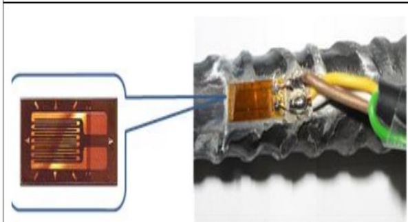
Figure 3: Detail of bonded and welding of electric gauge
