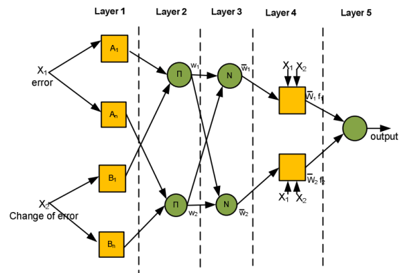
Fig5. An ANFIS structure.
