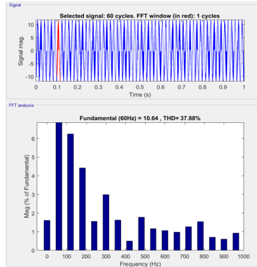
Fig11. (b)Grid Currents THD 37.88%
