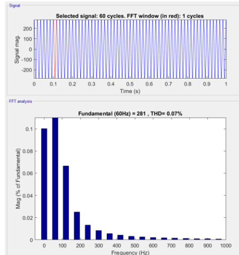
Fig14. (a) Inverter Voltage THD of 0.07%
