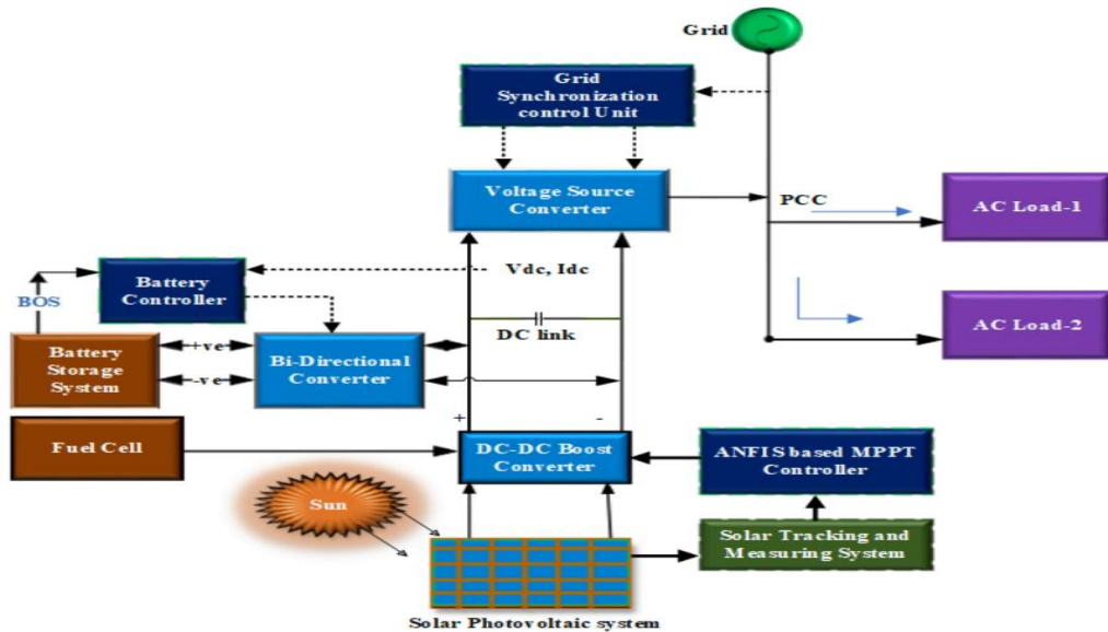
Fig1. Proposed hybrid system
