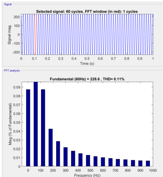
Fig11. Grid(a) Voltages
