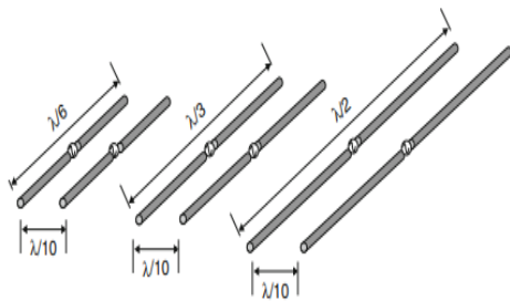
Fig. 4.1 Structures of fundamental MIMO dipole antennas
