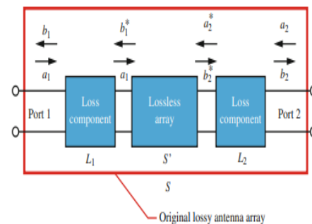
Fig. 2 Correlation coefficient calculation from S-parameters and radiation efficiency
