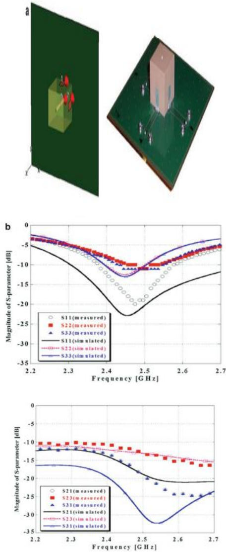
Fig.5.1 (a) Compact 3-port DRA MIMO antennas and (b) measured S-parameters
