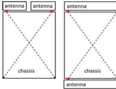
Fig. 6.3 Diagonal chassis mode in mobile terminals
