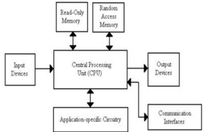
Fig: basic building blocks of Embedded System
