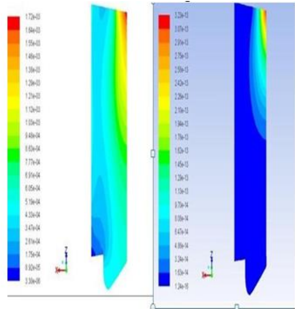
Fig. 5. NOx (85%-5-15%) Soot(90%-10-10%)contour
