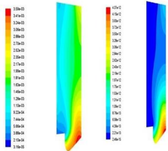
Fig. 4. NOx and soot contour-single injection
