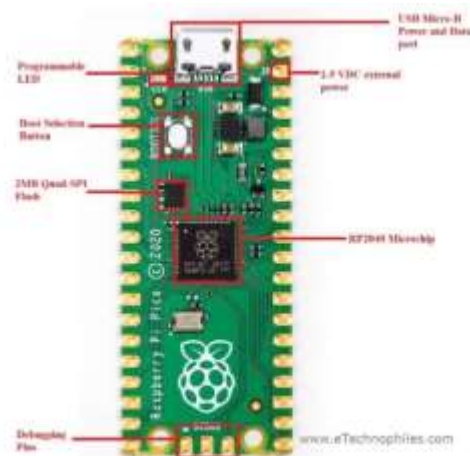
Raspberry Pi PICO Board Layout
