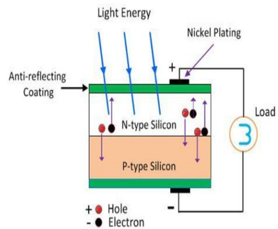
Fig.1: Solar cell
