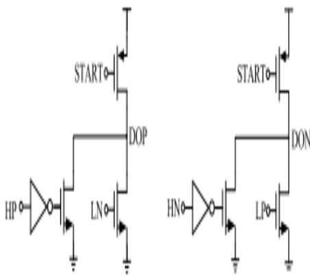
Fig. 7. Circuit to obtain the final comparison result. extra transistors M17–M20 into Fig. 6 to effectively reduce this disturbance.
