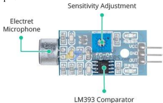
Fig 3: Sound Sensor
