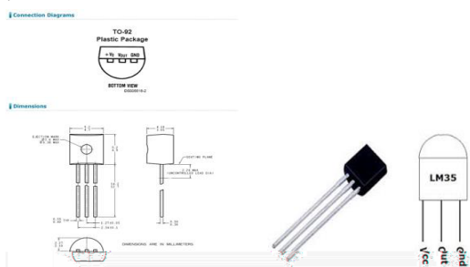
Fig4: Temperature sensor
