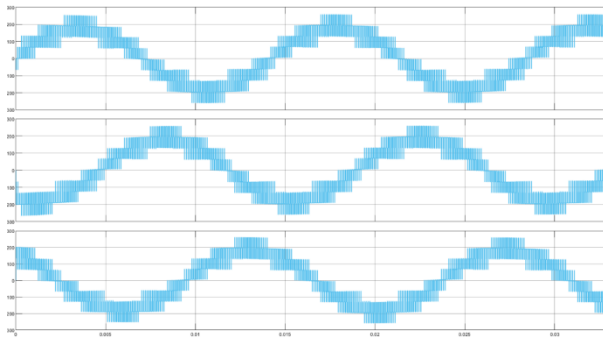
Stator Line Currents
