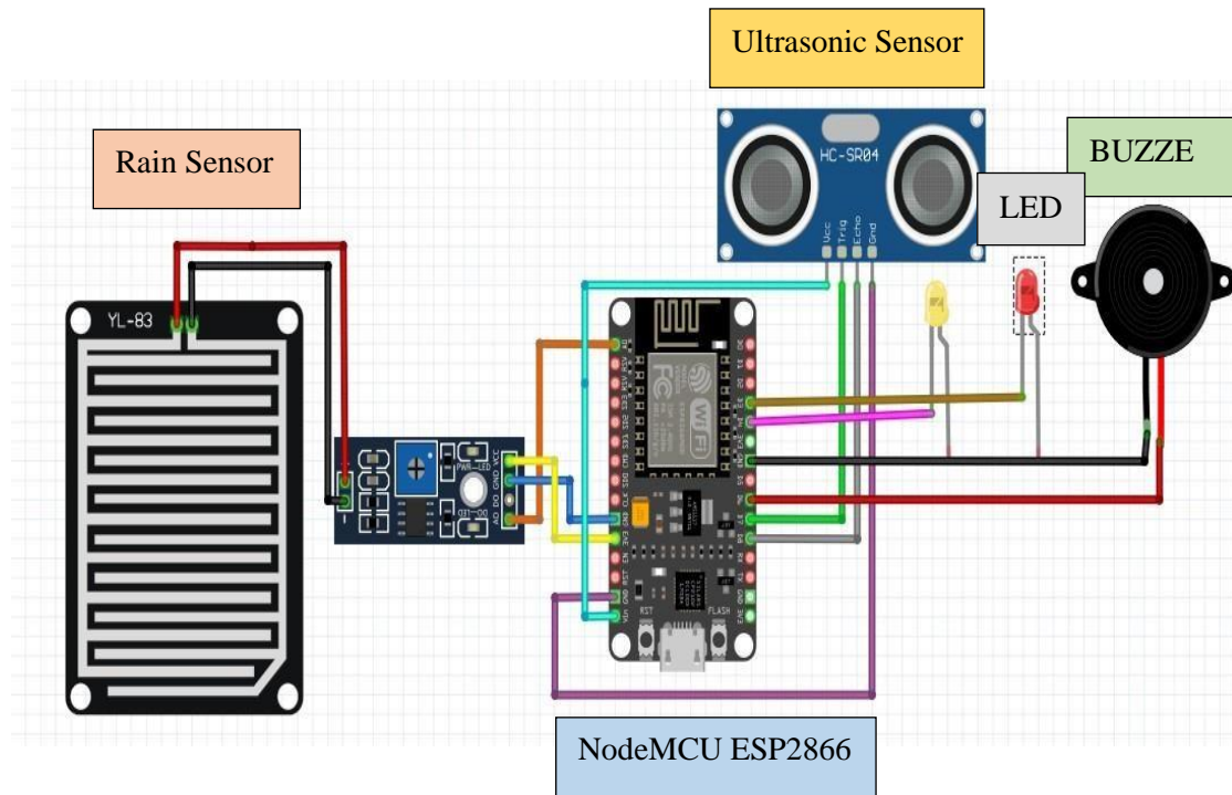
Fig - 3.2 Circuit Diagram of Proposed System
