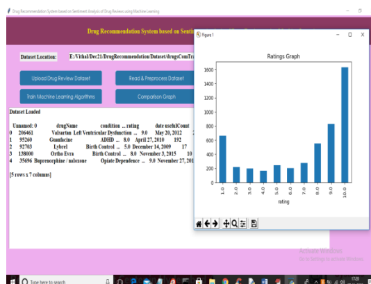
Fig.3. Ratings Graph
