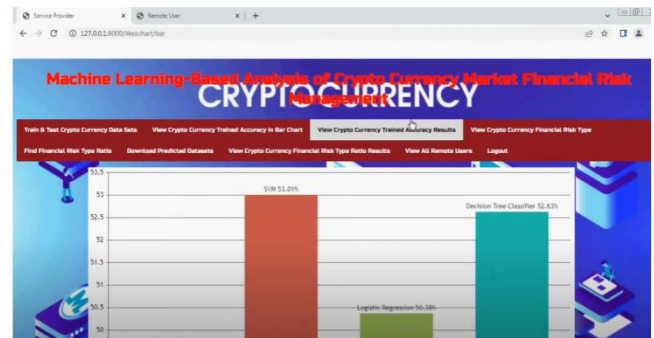
Fig.6. graph analysis.
