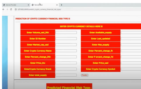
Fig.5. prediction values.
