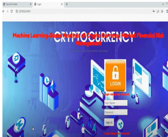
Fig.3. student registration.
