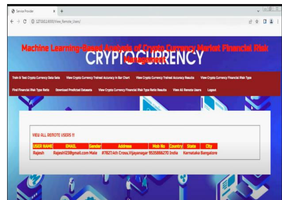
Fig.1. Home page.
