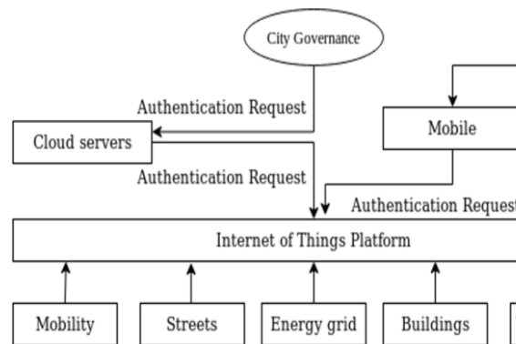
System architecture
