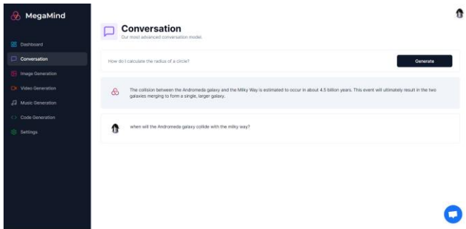
Fig. 3. Conversational AI
