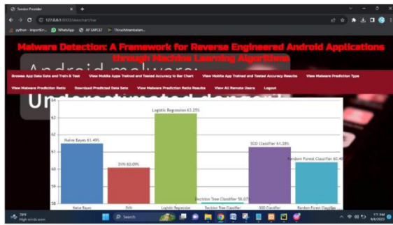
Fig.4 training and tested accuracy
