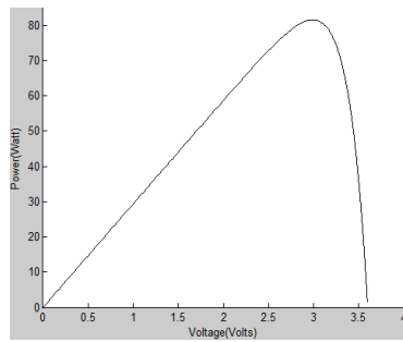
6*4 photovoltaic array
