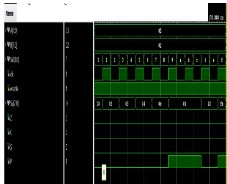
Fig 4 Simulation of ALU in vivado
