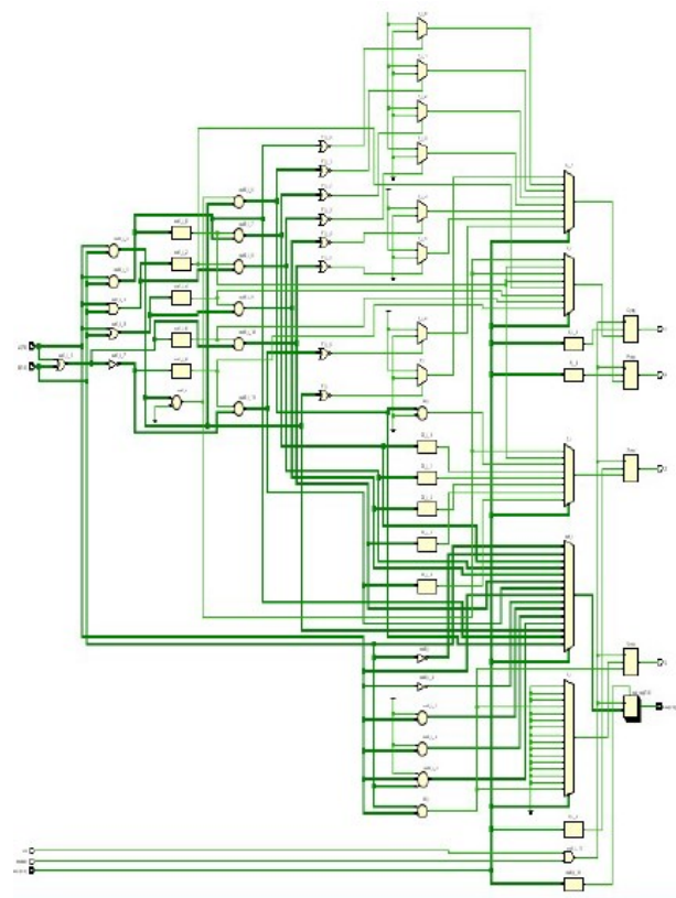
Fig 5 RTL Schematic of normal ALU
