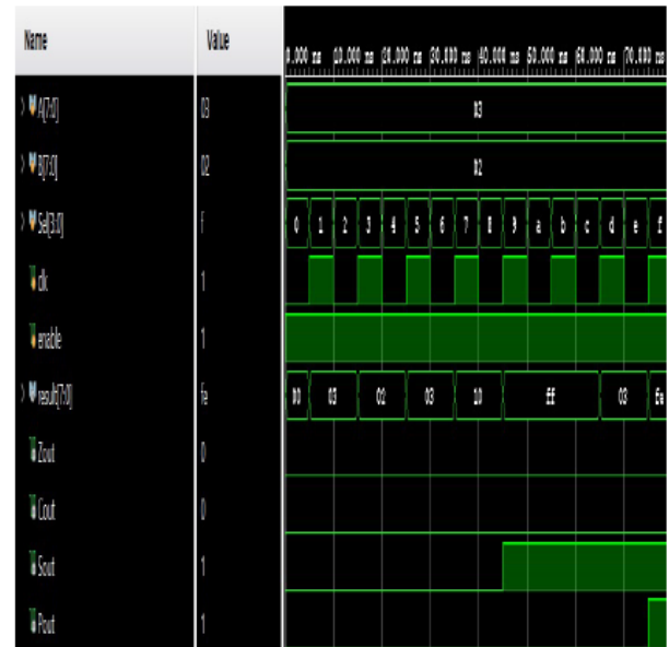
Fig 7 Simulation of modified ALU in vivado
