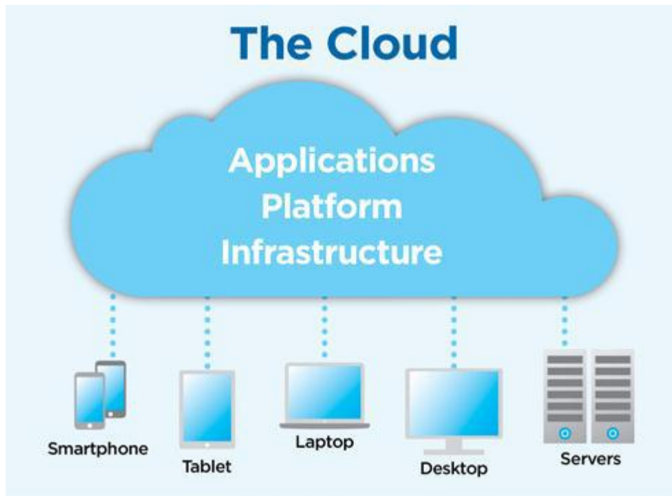
Figure 1: Cloud Architecture
