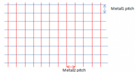
Figure 1 : Routing Grids
