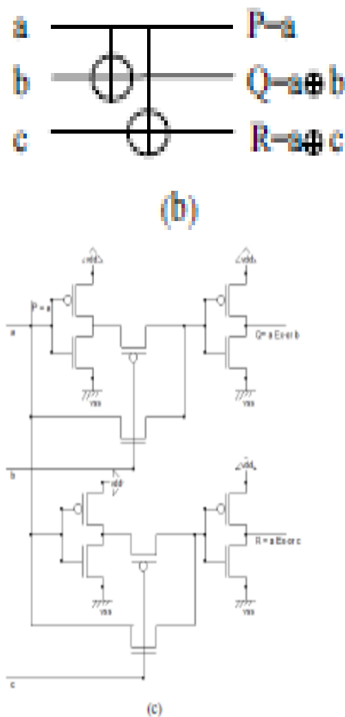
Fig.4.3.1: Reversible Feynman double gate (a) Block diagram (b) Quantum equivalent realization (c) Transistor realization
