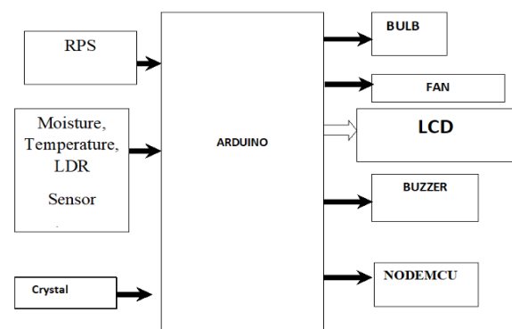
BLOCK DIAGRAM:
