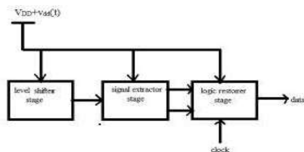
Fig. 1 Block Diagram of Proposed Power Efficient CMOS PLC Receiver
