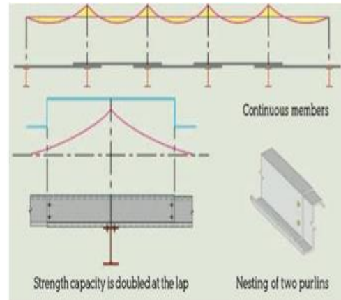
Fig – 5: Image courtesy: (Mr. Roshan S Satpute, et. al “Building Design Using Cold Formed Steel Section”)
