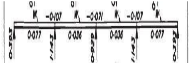
Fig - 4 Bending Moment and reaction Co-efficient - Equal span continuous beams – UDL as per Steel Designer's Manual – AISI
