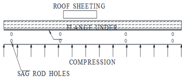
Fig - 8: Bottom flange of the purlin under compression
