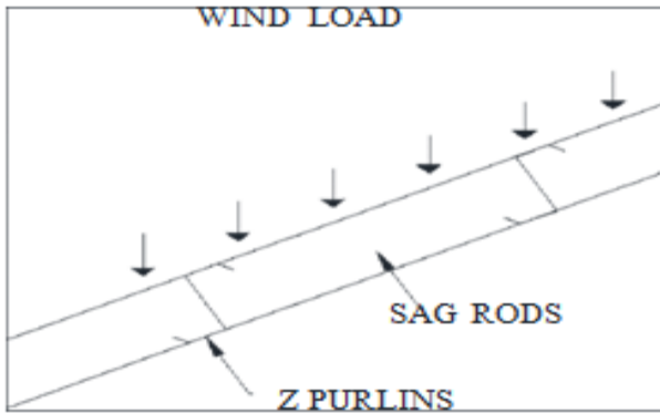
Fig - 6: Z Purlins under gravity load
