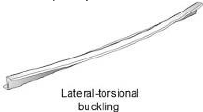
Fig - 10: Lateral torsional buckling of Z section
