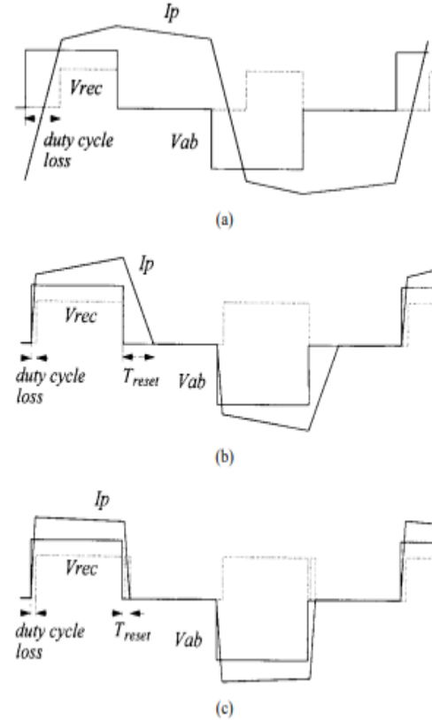
Fig. 4. Comparison of the simplified waveforms of primary voltages and currents and secondary rectifier voltages. (a) ZVS PWM converter. (b) ZVZCS PWM converters [7], [8]. (c) Proposed converter.
