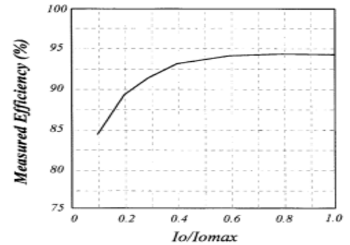
Fig. 14. Measured efficiencies.
