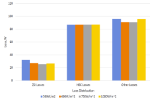
Fig. 9. Loss distribution chart for the MZSI topology for a fixed charging power P_B=3.3 kW at 25 ^{\circ} C, under varying irradiation
