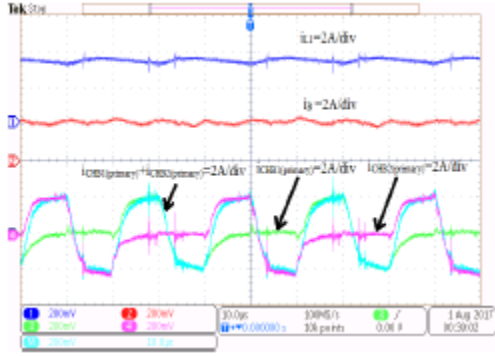
Fig. 13. Experimental setup waveforms for the Inductor current(top), charger output current(middle) and the primary currents of the split charger(bottom) From equation (22), at D_0=0.2 , for an input current i_{PV}=3.82 A and fixed HBC output current i_B=2 A, the ZSI AC output current i_g is calculated to be 2.87 A. Fig.13 shows the the inductor current i_{L1} , the battery current i_B and the split primary current i_{CHB1} and i_{CHB2} and the total primary current. Each of the primary operate alternately. The total primary current is a high frequency alternating current of f_{HBC}=50 kHz. From Fig. 13 and Fig. 14, the charger output current is maintained at 2 A using a Chroma Programmable AC/DCElectronics Load(Model 6304). The PV input current is maintained at 3.82 A using a Magna-power LXITM solar emulator. The output grid current is observed to be 2.66 A. Fig. 15 shows the experimental setup for the proof of concept. The lower values of the output current is a result of the losses in the circuit. The practical PI values for the ACside current control was K_P=0.03 and the battery loop was K_{PB}=0.0003 and K_{IB}=0.09 and the input PV current loop were K_{Pin}=0.005 and K_{Lin}=2 .
