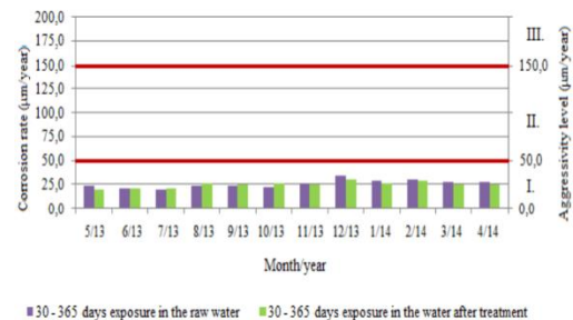
Raw water corrosion vs treated water corrosion velocity data over a 30-365 day period are shown in Fig. 6.
