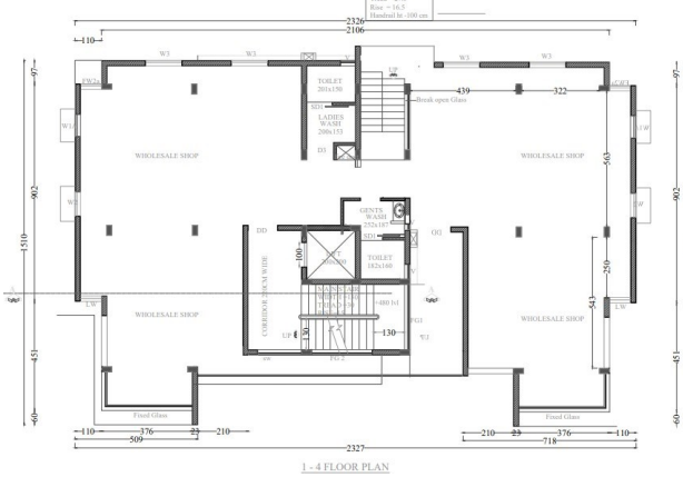
Fig 3.2. 1-4 Floor Plan
