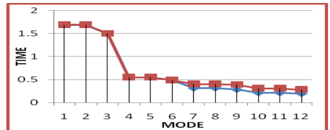
Fig.11. comparison between two building Modal Periods for 15 storey.
