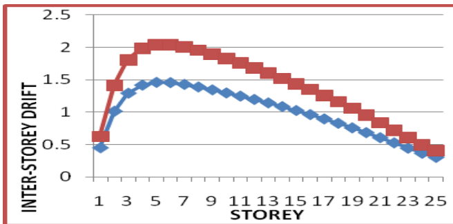
Fig.20. Inter storey drift for 25 storey building.
