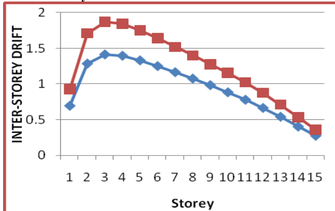
Fig.19. Inter storey drift for 15 storey building.
