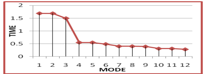
Fig.10. Modal Periods for 15 storey with TMD.
