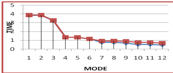
Fig.13. comparison between two buildings in Modal Periods for 35 storey.
