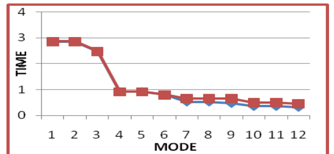
Fig.12. comparison between two building Modal Periods for 25 storey.
