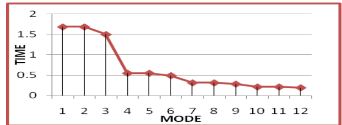
Fig.9. Modal Periods for 15 storey without TMD.
