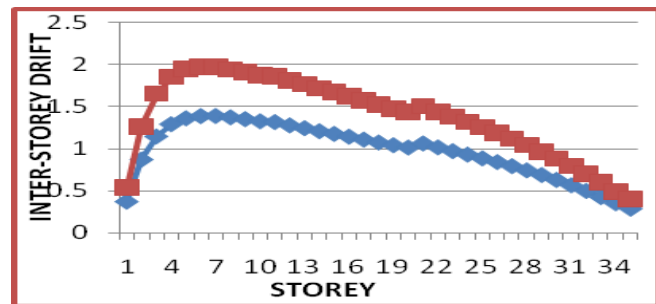
Fig.21. Inter storey drift for 35 storey building.
