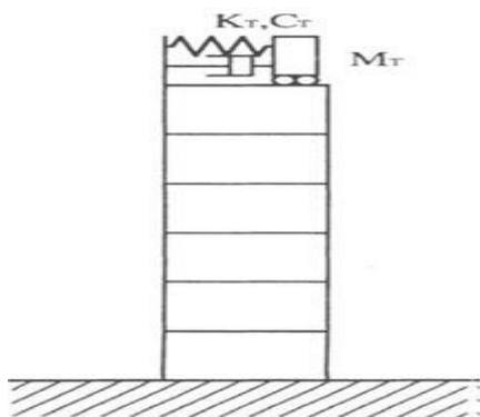
Fig. 4. Tuned mass damper on a structure.
