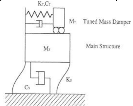
Fig. 5. 2-DOF modeling of main structure and tuned mass damper system.
