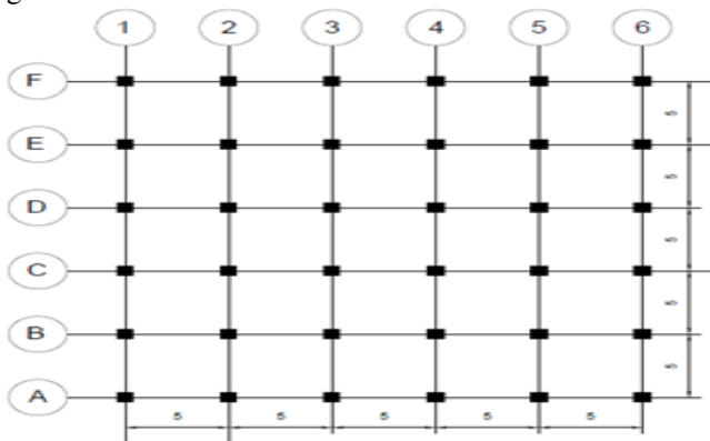
Fig.6. Plane of the models.
