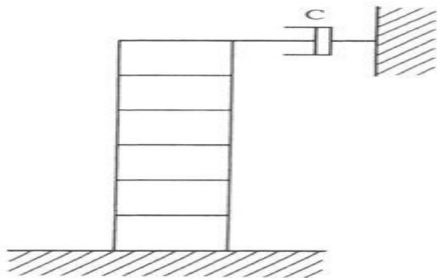
Fig. 3. Viscous damper with fixed reaction wall.
